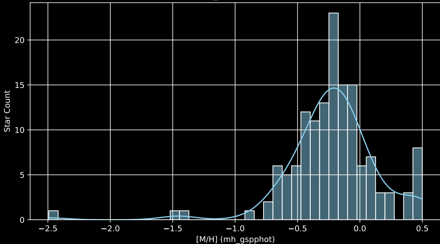
APOGEE DR17 Field: [052-33_MGA [M/H] (mh_gspphot) (n= 142)
