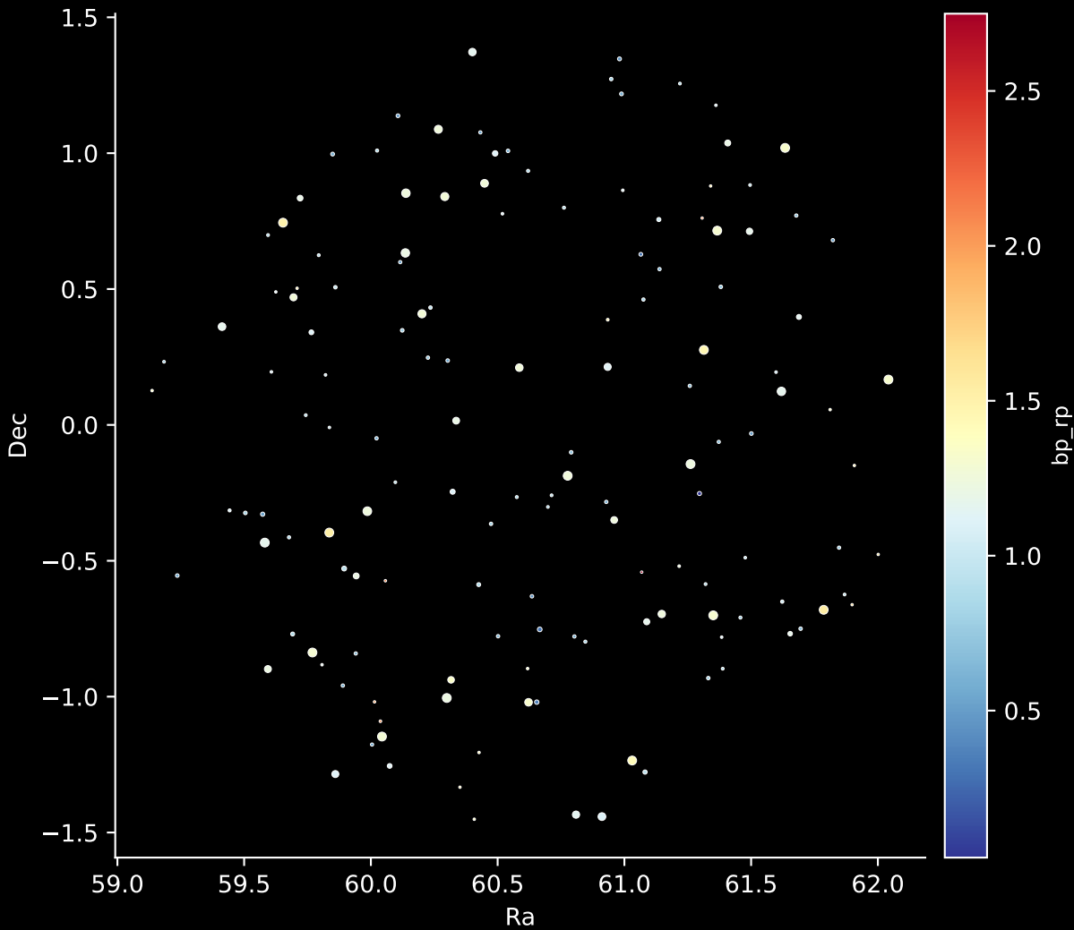
APOGEE DR17 Field: [052-33_MGA] Stars: 144
