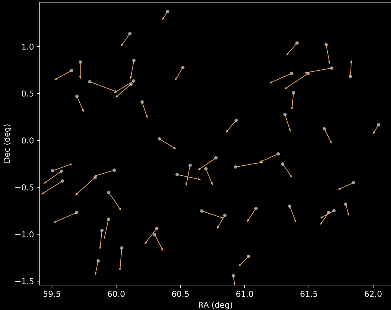
APOGEE DR17 Cluster 3 Proper Motion Vectors (n=53)
