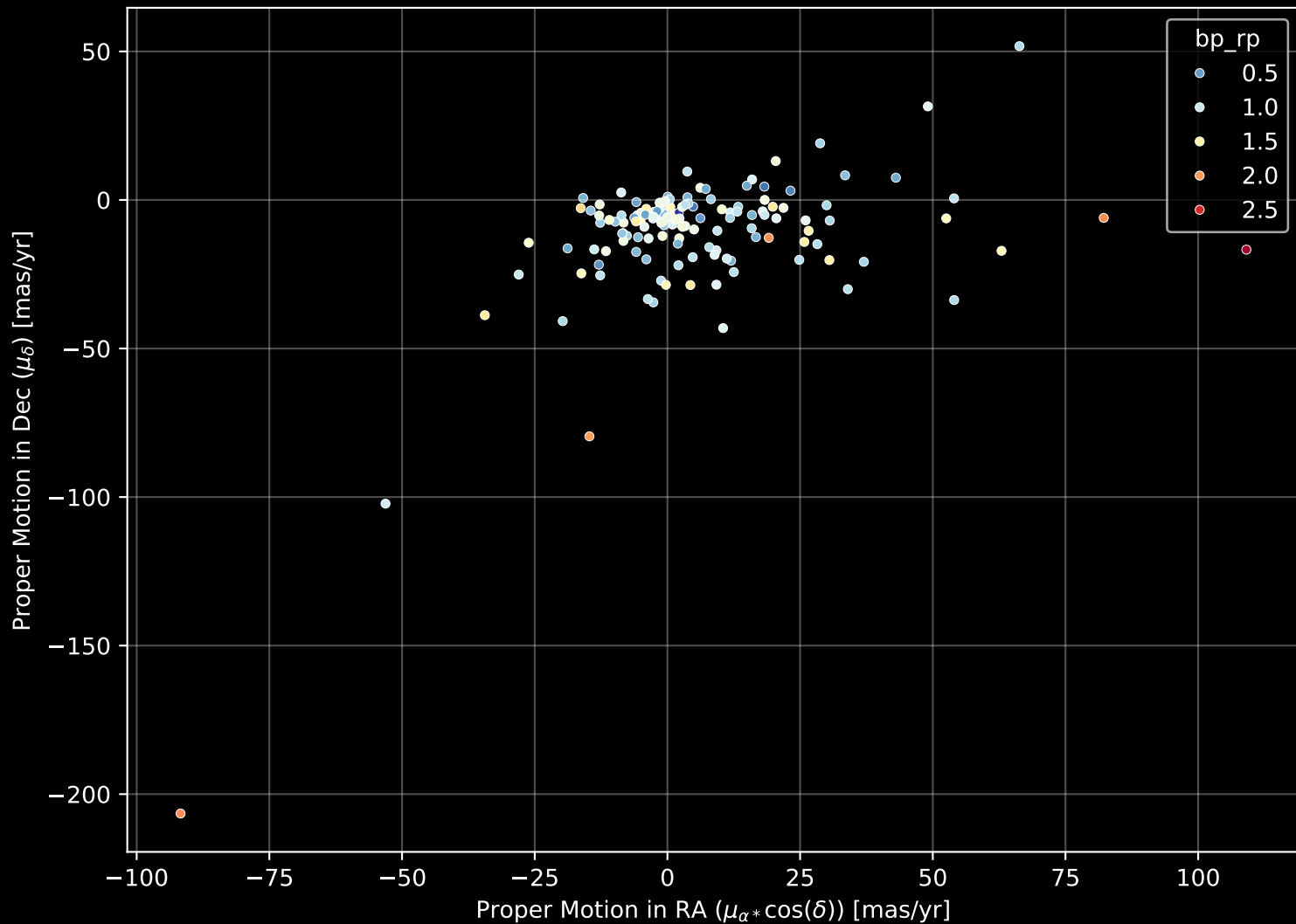
APOGEE DR17 Field: [052-33_MGA] Proper Motion Diagram (n= 144)
