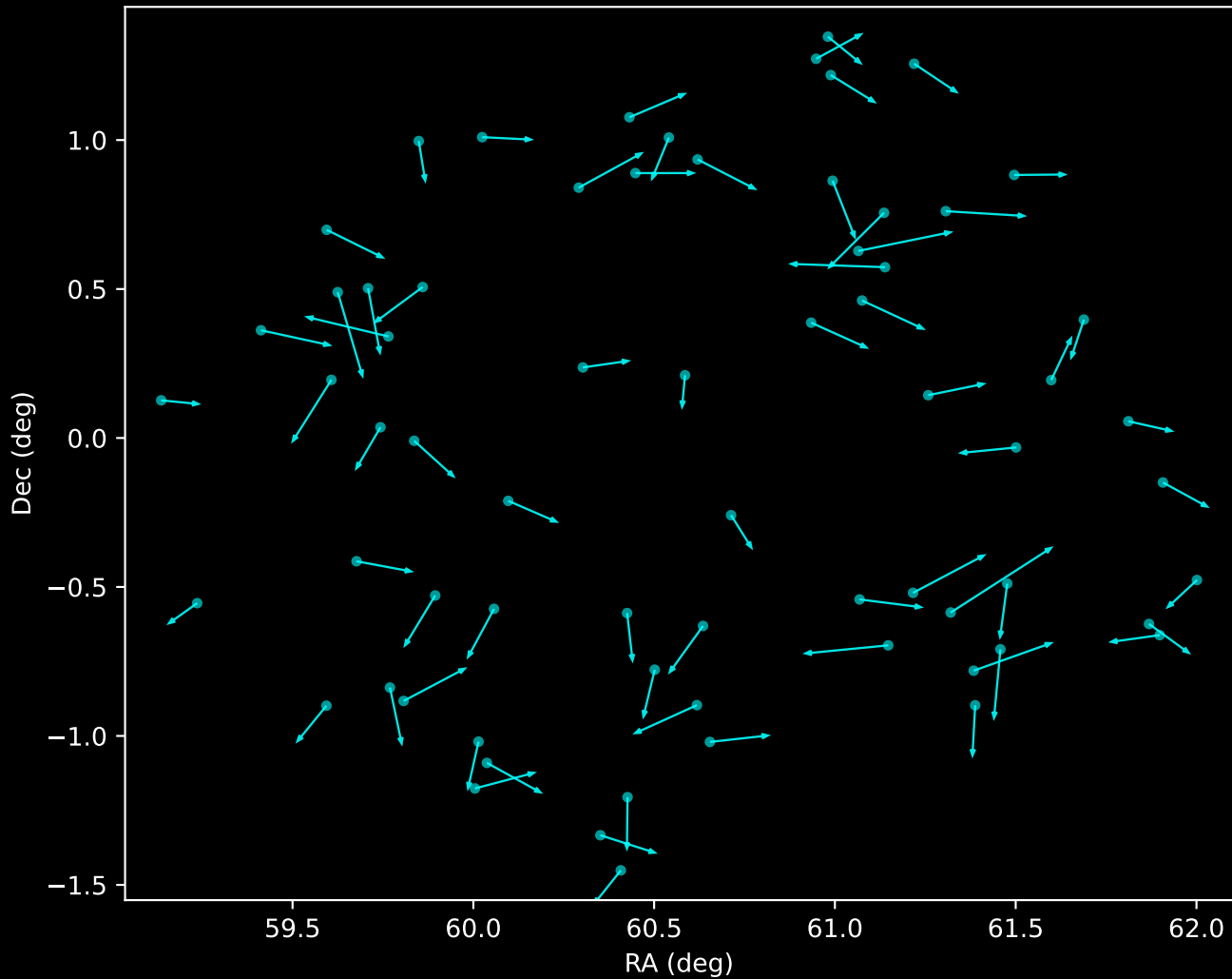
APOGEE DR17 Noise Stream Proper Motion Vectors (n=68)
