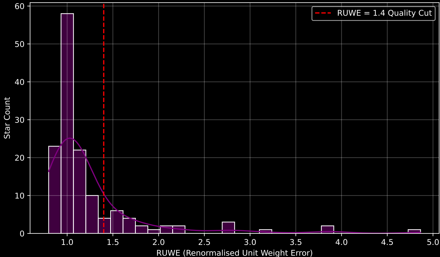
GAPOGEE DR17 Field [052-33_MGA] RUWE Distribution (n= 141)
