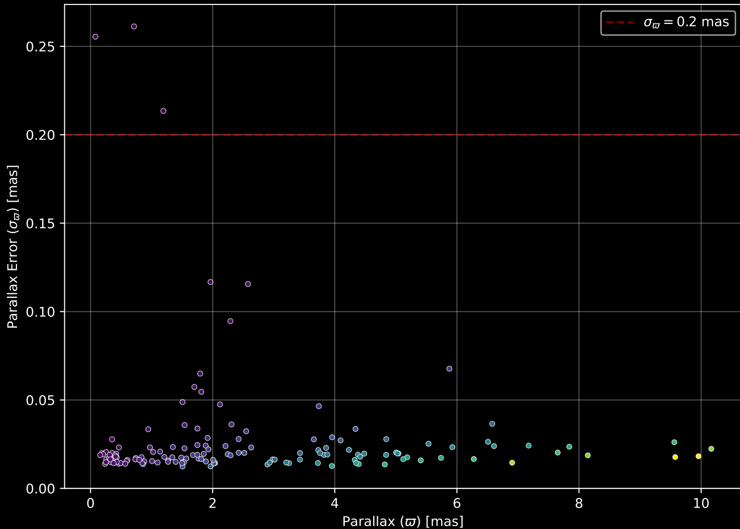
APOGEE DR17 Field: [052-33_MGA] Parallax Quality (n= 144)
