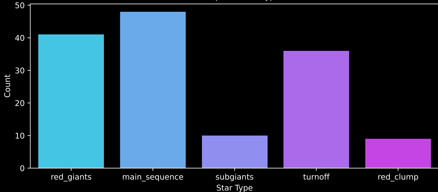
APOGEE DR17 Field: [052-33_MGA] Count plot of Star Type
